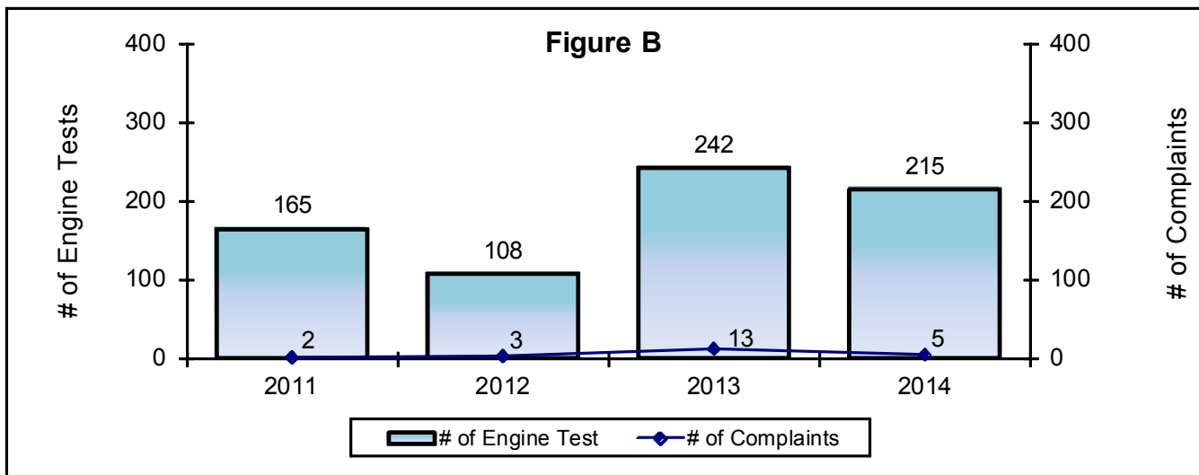
Figure B: Correlation between engine testing and engine testing related noise complaints (January – December 2011-2014)
